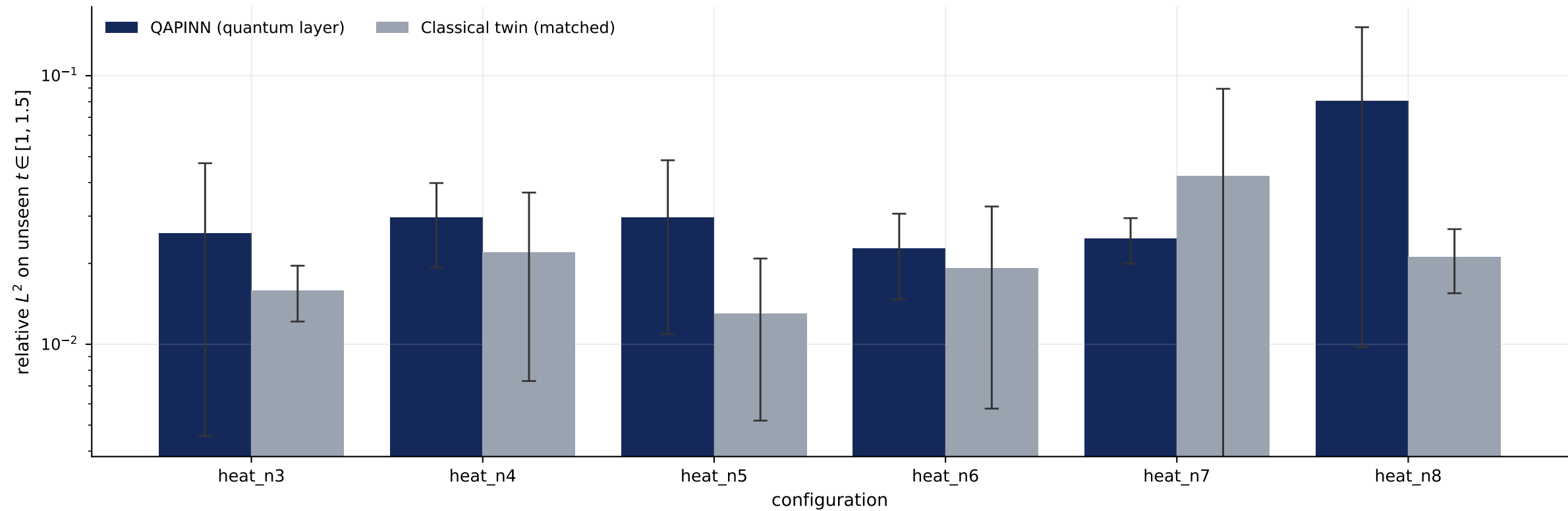
Generalization beyond training domain (mean \pm s.d., 3 seeds)
